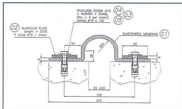
Taiwan High Speed Rail – longitudinal expansion joint
