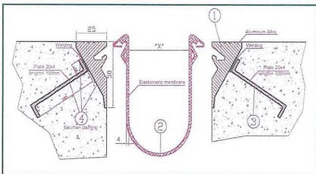
Taiwan High Speed Rail – transversal expansion joint
